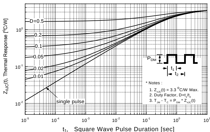
Figure 10. Transient Thermal Response Curve
