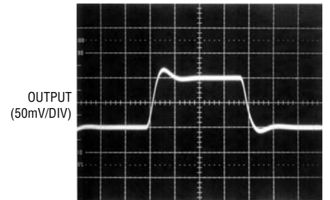
Small-Signal Transient Response (IS = 300μA per Amplifier)
