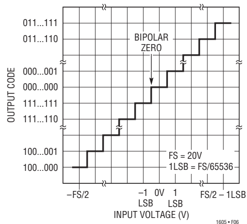
Figure 6. LTC1605 Bipolar Transfer Characteristics
