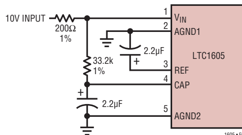
Figure 4. \pm 10V Input Without Trim
