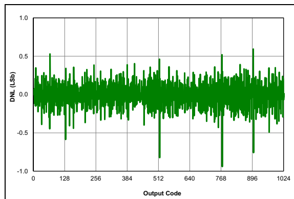
FIGURE 29-64: ADC 10-bit Mode, Single-Ended DNL, V_{DD} = 3.0V , T_{AD} = 4\text{ }\mu S , 25^\circ C .
