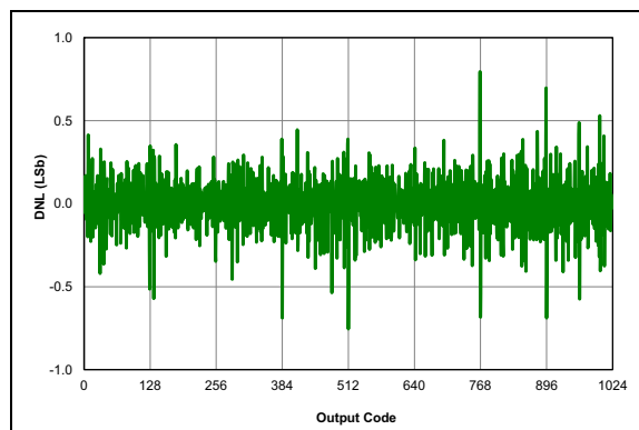
FIGURE 29-63: ADC 10-bit Mode, Single-Ended DNL, V_{DD} = 3.0V , T_{AD} = 1\text{ }\mu S , 25^\circ C .
