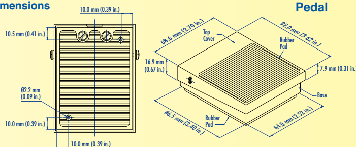
Pedal
