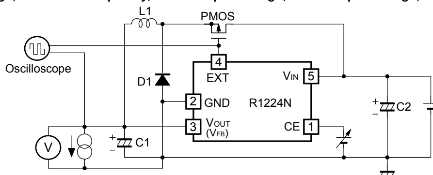
Supply Current 1
