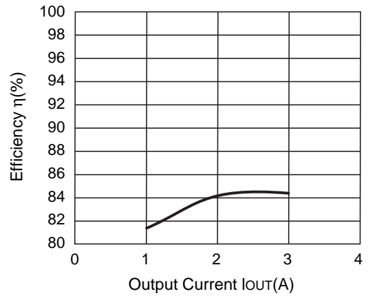
R1224N332M (V IN =18V)
