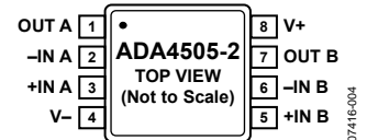
Figure 2. 8-Lead MSOP (RM-8)
