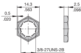
Knurled nut 3/8", 27-thread plastic (standard) Y 307 117 02
