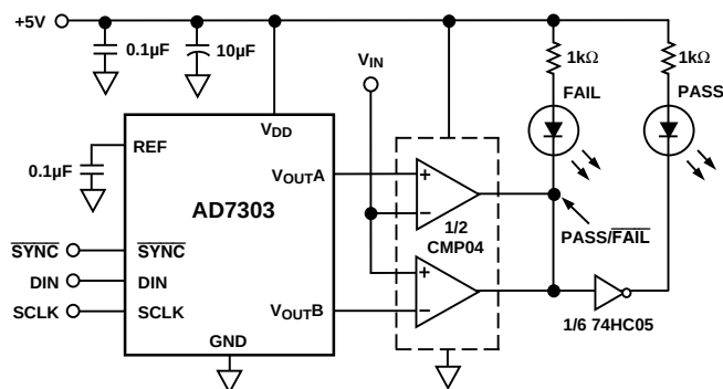
Figure 34. Window Detector Using AD7303
