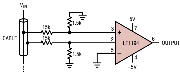
1% RESISTOR WORST-CASE CMRR = 22dB TYPICALLY = 38dB
