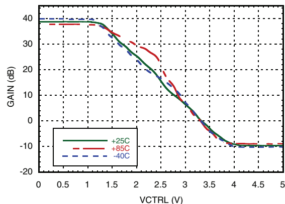
Gain vs. VCTRL @ 100MHz [2]
