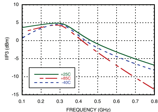
Input IP3 vs. Frequency over Temperature [1][3][5]
