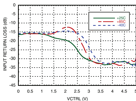
Input Return Loss vs. VCTRL @ 100MHz [1]
