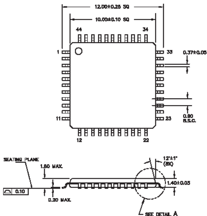
Figure 4-4. 44-Lead TQFP
