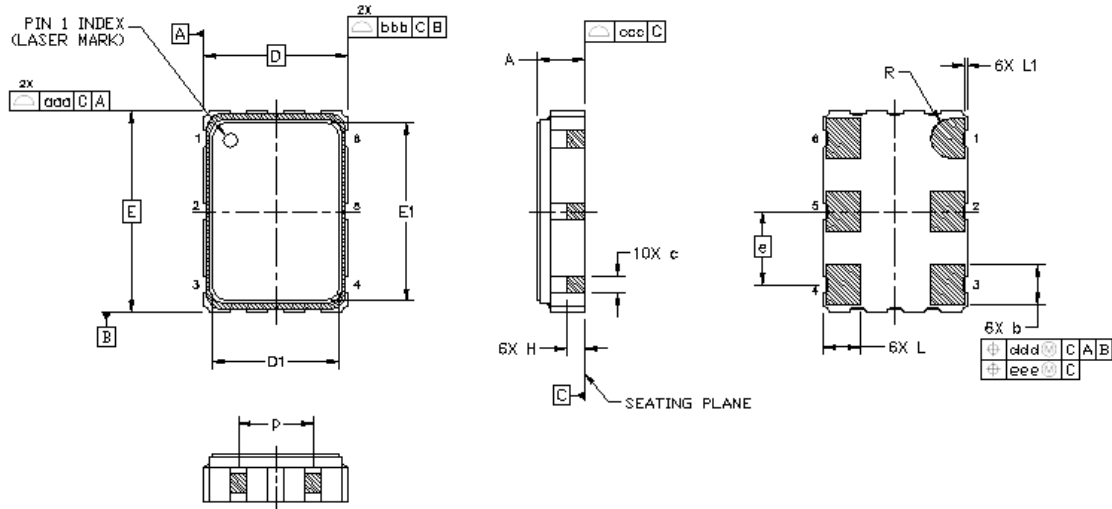
Figure 3. Si516 Outline Diagram
