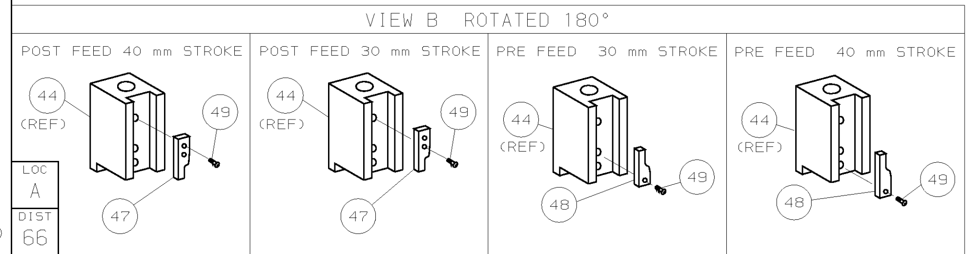
VIEW B ROTATED 180°
