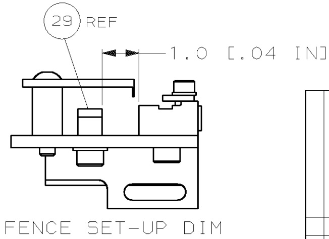
FENCE SET-UP DIM
