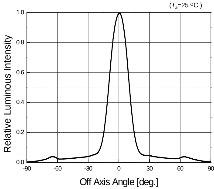
Radiation Diagram
