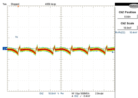
Fig. 5: Output Voltage Ripple, 35A load Ch 1 : V_o
