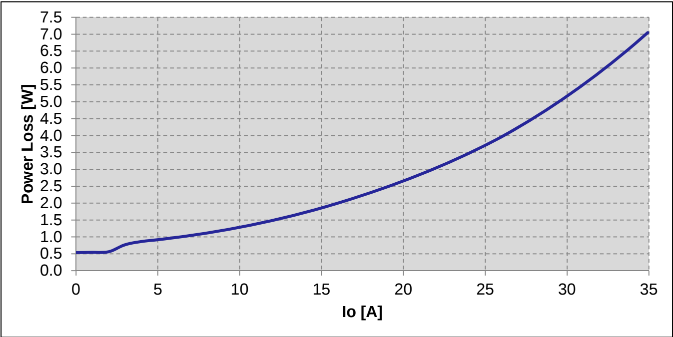
Fig.12: Power loss versus load current
