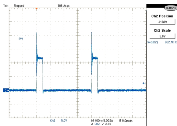
Fig. 6: Inductor node at 35A load Ch 2 :LX
