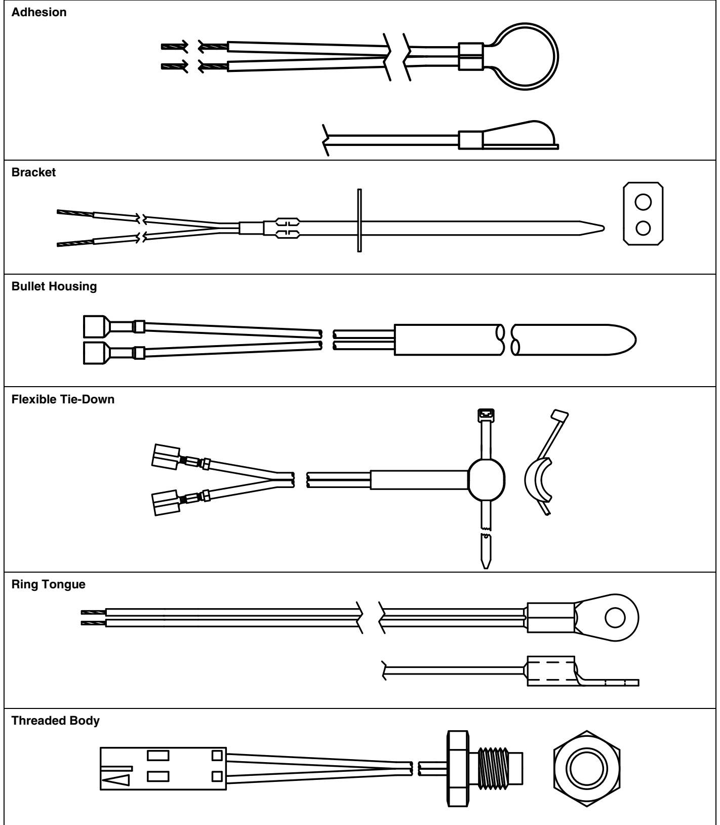
Figure 1. Mounting Methods
