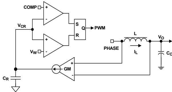
FIGURE 25. R3 MODULATOR
