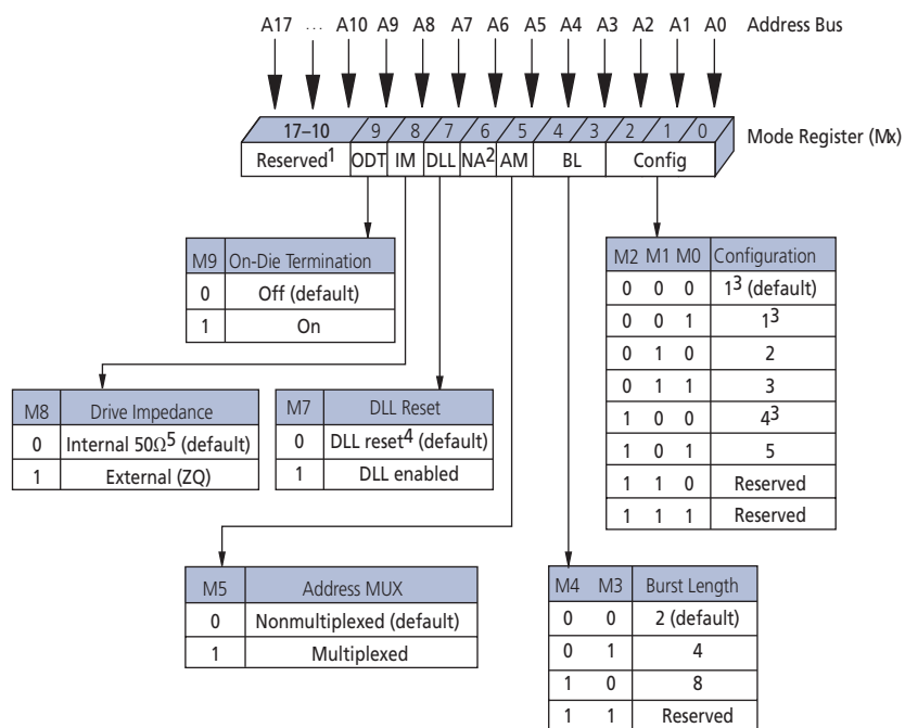
Figure 12: Mode Register Definition in Nonmultiplexed Address Mode
