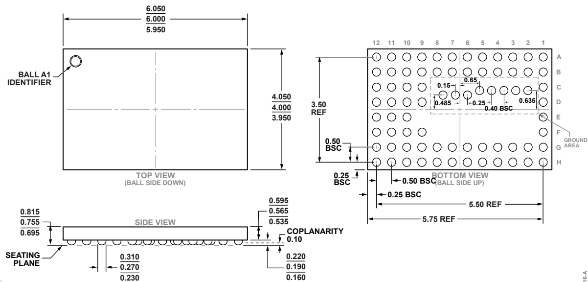
Figure 22. 75-Ball Wafer Level Ball Grid Array [WLBGA] (BF-75-1) Dimensions shown in millimeters
