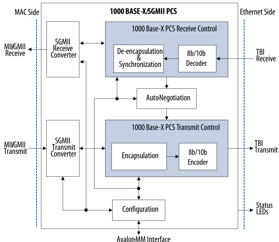
Figure 24. 1000BASE-X/SGMII PCS
