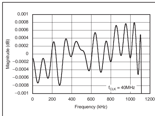
Figure 49. Passband Ripple
