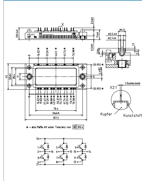
EconoPACK™ 2 A (shortpin)
