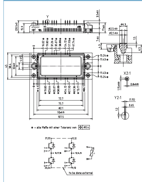
EconoPACK™ 2 B FourPACK
