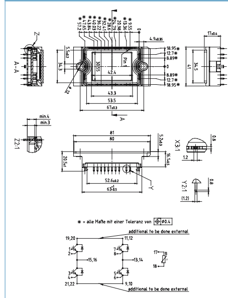
EconoPACK™ 1B FourPACK
