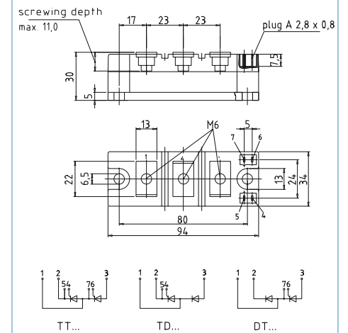
34 mm TP34
