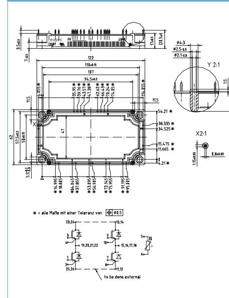
EconoPACK™ 3 B FourPACK
