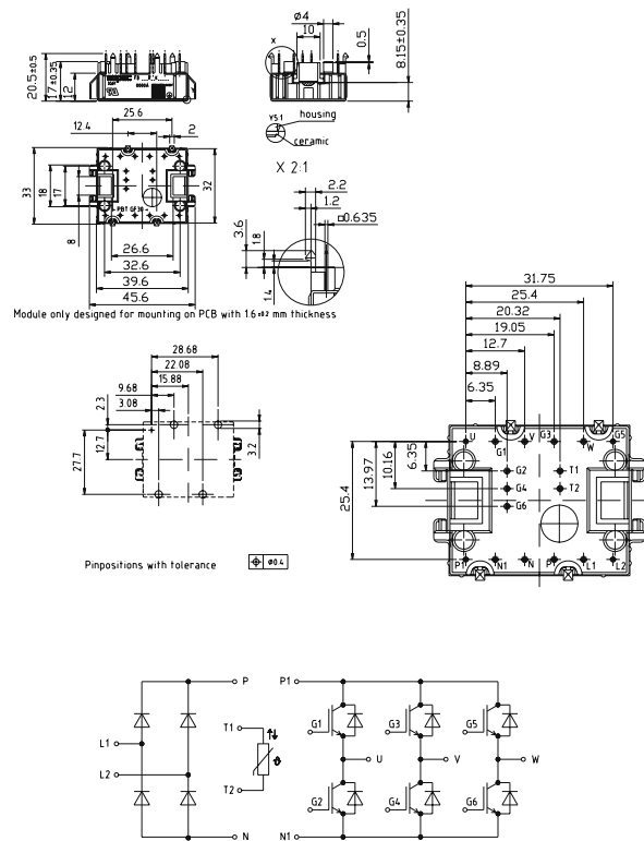
EasyPIM™1
