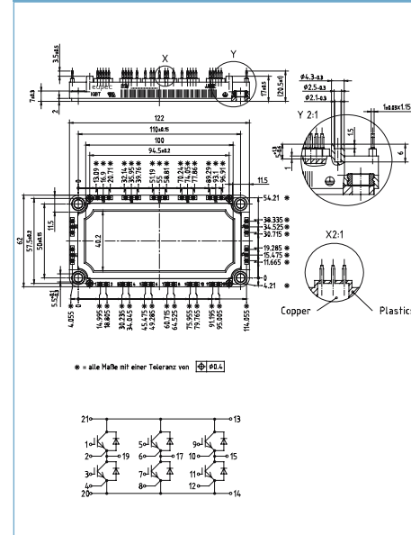
EconoPACK™ 3 A
