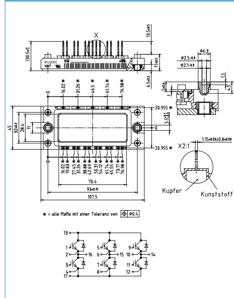
EconoPACK™ 2 A (longpin)
