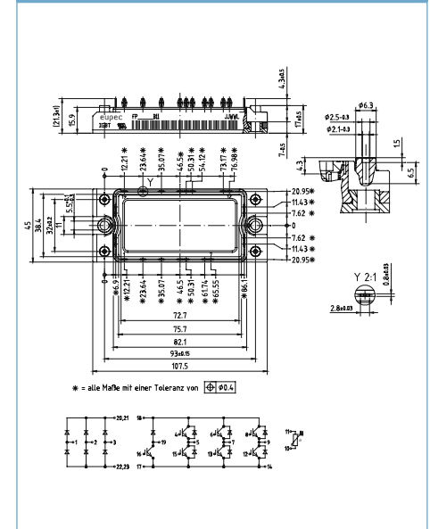
EconoPIM™ 2B PressFIT
