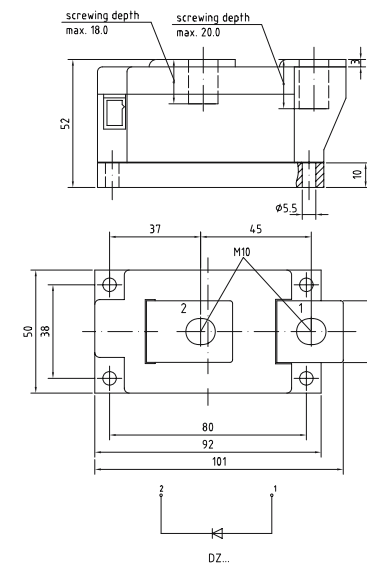
70 mm DP70
