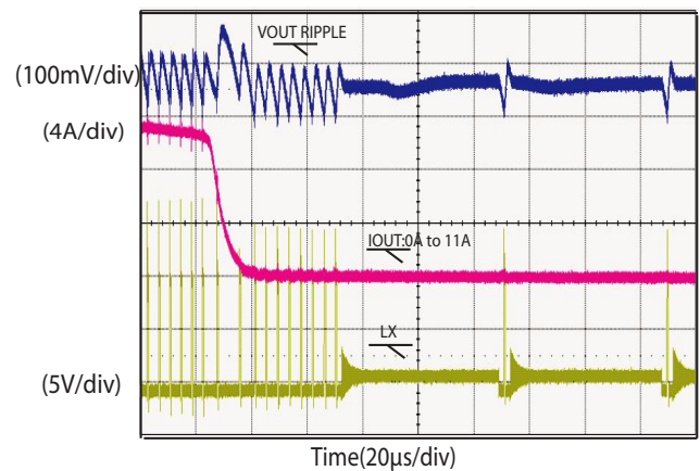
Transient Response - P-Save Load Falling ( V_{DD} = 5\text{ V} , V_{IN} = 12\text{ V} , V_{OUT} = 1.5\text{ V} , I_{OUT} = 11\text{ A to } 0\text{ A} , SiC401A, dI/dt = 1\text{ A}/\mu\text{s} )
