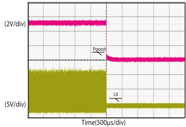
Over Temperature Shutdown at 133.4 °C ( V_{IN} = 12\text{ V} , V_{OUT} = 1.5\text{ V} , I_{OUT} = 0\text{ A} , LDO Mode, SiC401B)
