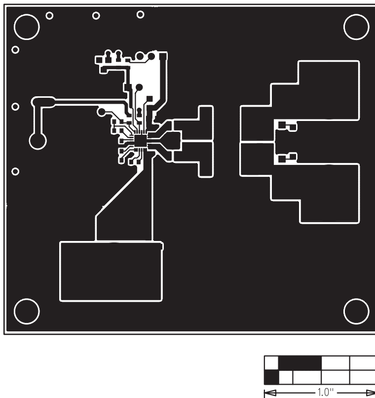
Figure 3. MAX9737 EV Kit PCB Layout—Component Side
