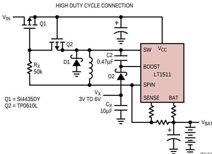
Figure 11. Replacing the Input Diode
