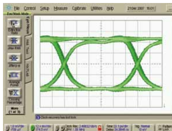
Eye Diagram
