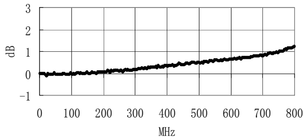
Phase Balance
