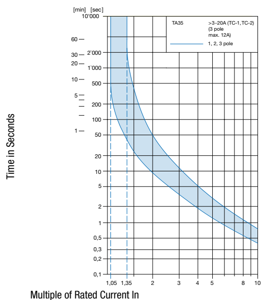
Tripping Characteristics I_n 3\text{ -}20\text{ A}
