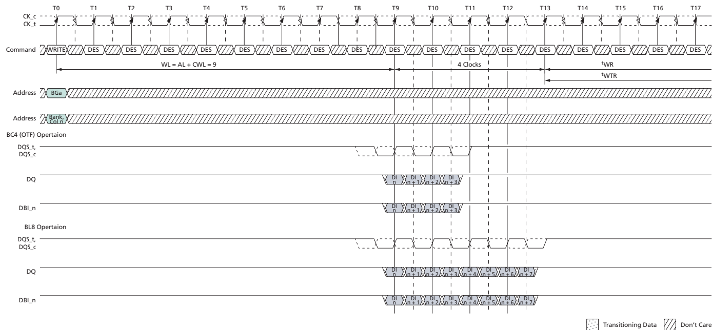
Figure 193: WRITE (BL8/BC4-OTF) with 1 st CK Preamble and DBI
