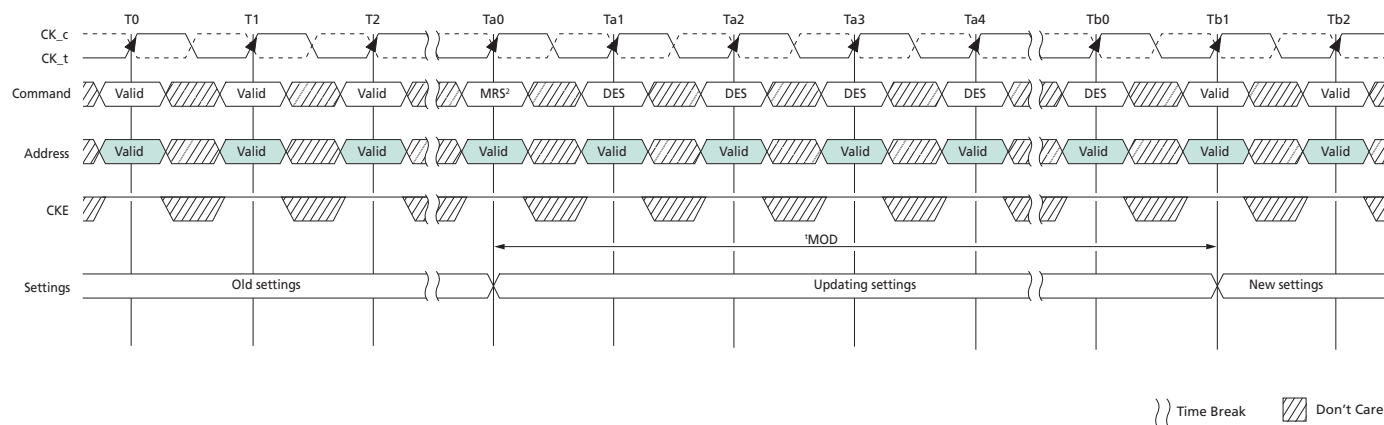
Figure 18: t^{\text{MOD}} Timing
