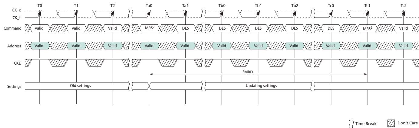
Figure 17: t^{\text{MRD}} Timing
