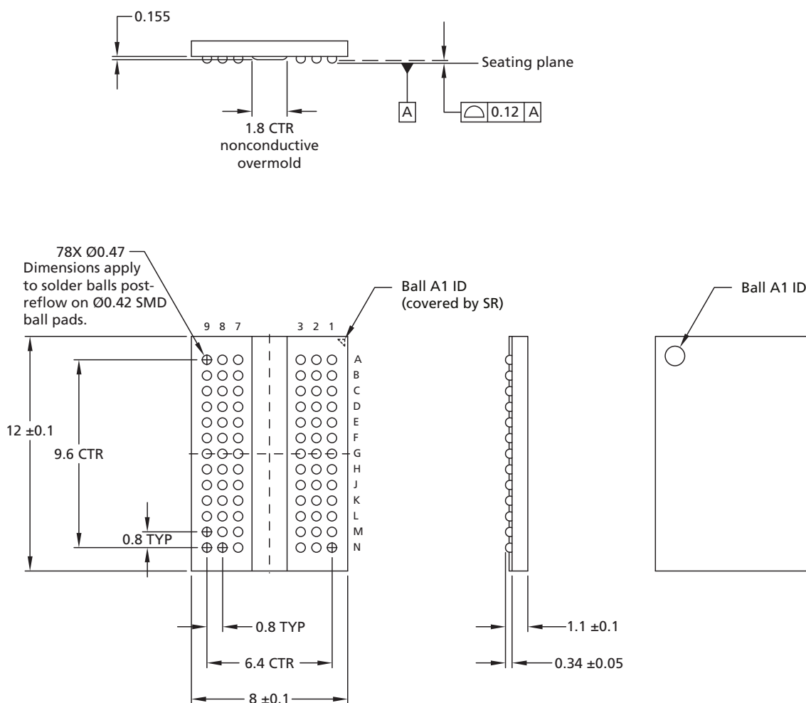
Figure 9: 78-Ball FBGA – x4, x8 "WE"
