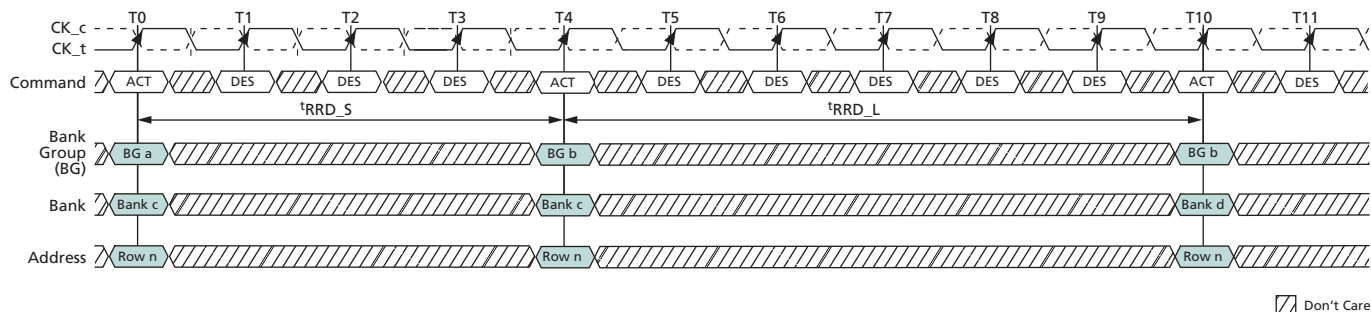
Figure 81: t_{RRD} Timing
