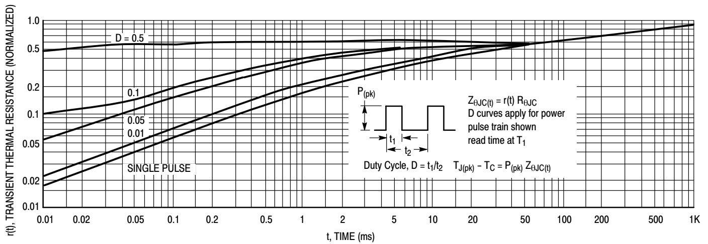
Figure 5. Thermal Response
