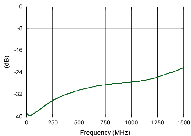
Input Return Loss, 75 \Omega (pin 3)
