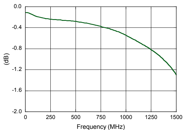
Insertion Loss (pin 3-4)
