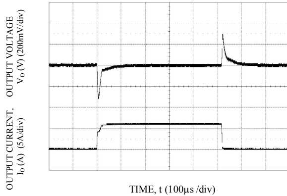
Transient Response to Dynamic Load Change from 0% to 50% to 0%. V_o=1.2V
