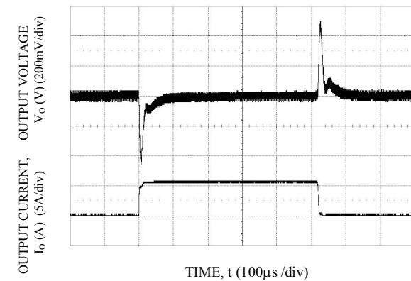
Transient Response to Dynamic Load Change from 0% to 50% to 0%. V_o=5.0V
