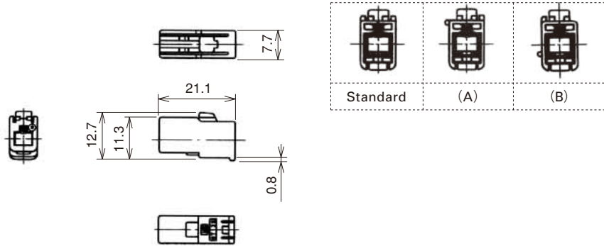
Retainer assembled
