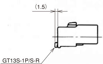
Retainer assembled
