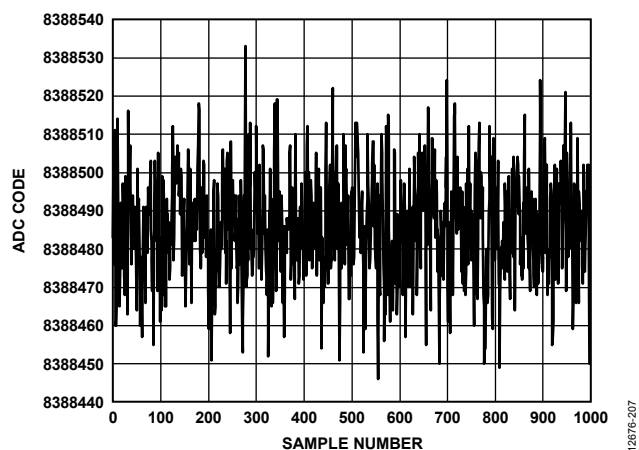
Figure 7. Noise (Analog Input Buffers Disabled, V_{REF} = 5 V, Output Data Rate = 31.25 kSPS)
