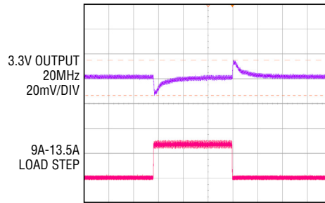
Figure 4. Measured Channel 1, 9A-13.5A Load Transient ( V_{IN} = 12V , V_{OUT1} = 3.3V )
