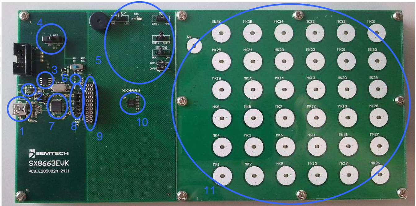
Figure 7: SX8663EVK Board Picture
