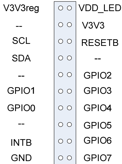
Figure 9: Header
