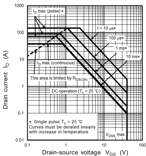
Fig. 8.16 Safe Operating Area (Guaranteed Maximum)
