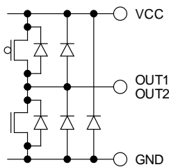
Figure 39. OUT1 / OUT2 (SOP8/HRP7)
