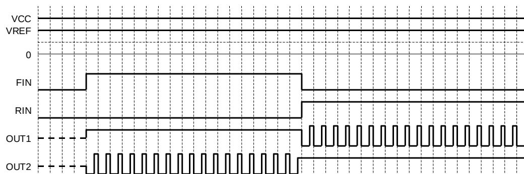
Figure 35. VREF Control Operation (Timing Chart)
