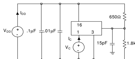
Figure 3. OUT1, OUT2, RDATA and RCLK Test Conditions (25 \pm 5 ^{\circ}C )
