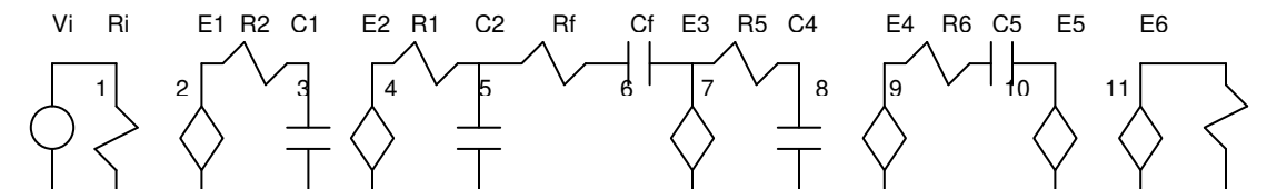
Figure 7. SPICE Model
