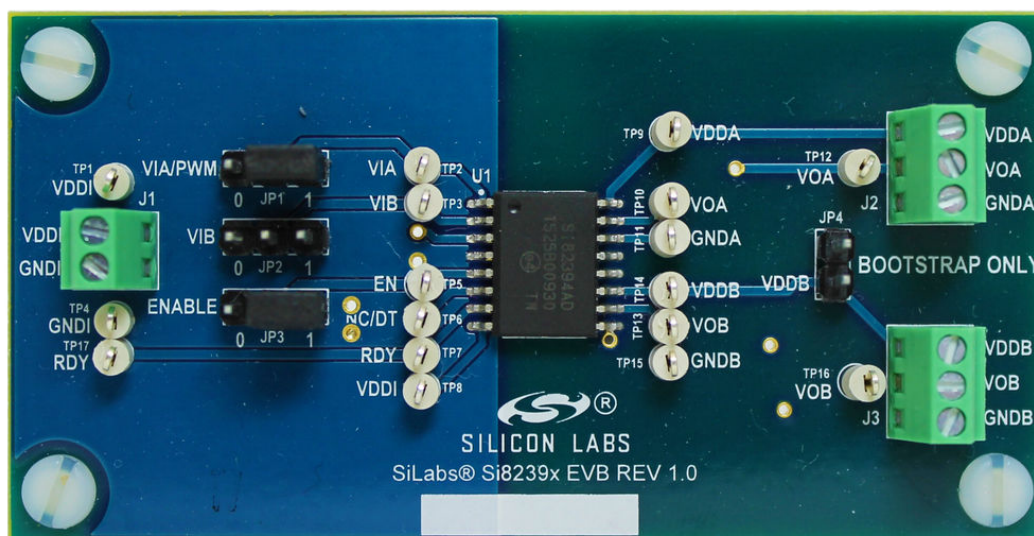
Figure 1.1. Si8239x Evaluation Board Front
