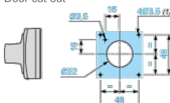
Door cut-out
