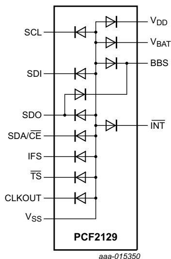
Fig 39. Device diode protection diagram of PCF2129
